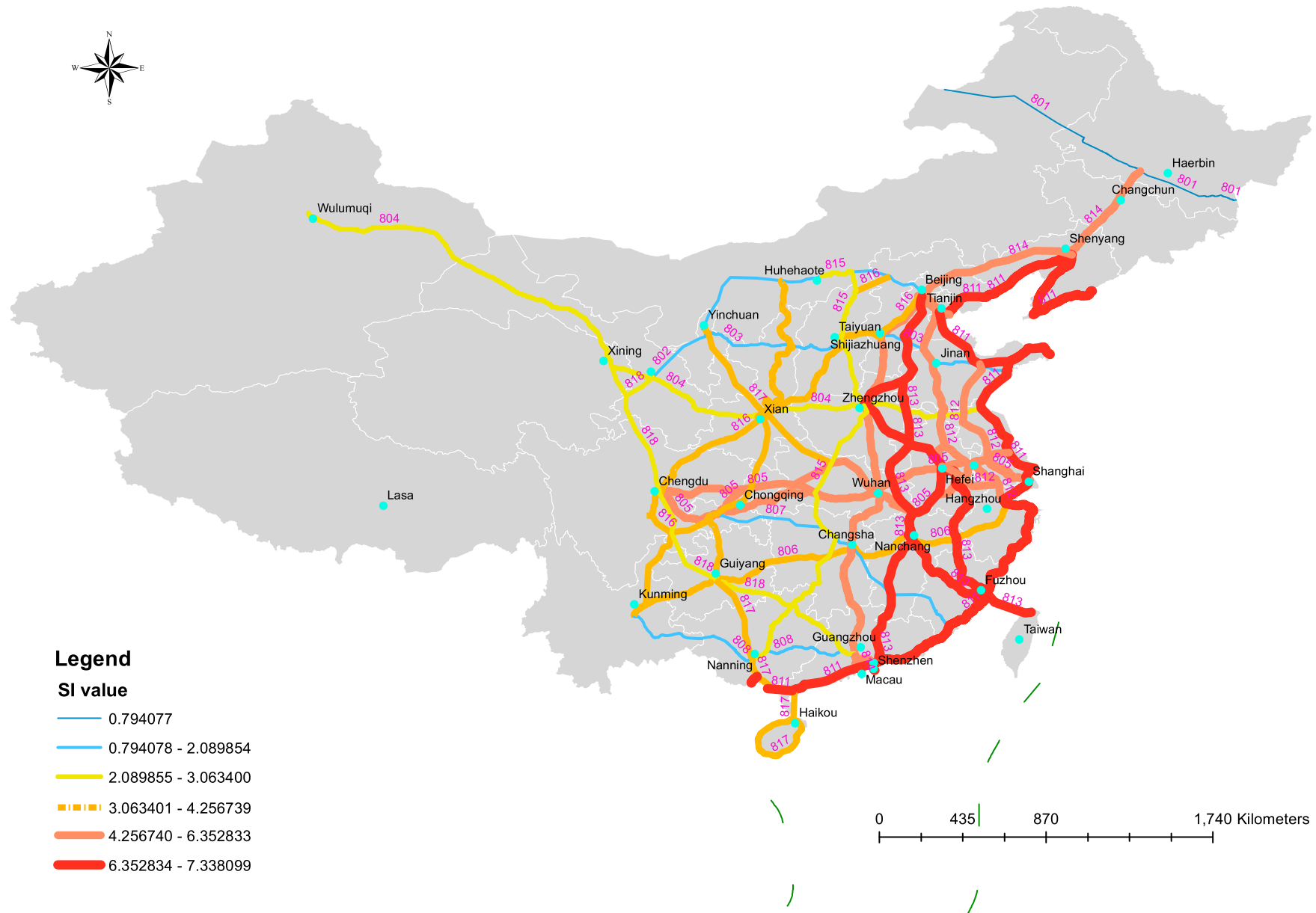
Fig. 4. Proportional symbols with graduated colors according to SI value of the eight-horizontal and eight-vertical HSR corridors. (For interpretation of the references to colour in this figure legend, the reader is referred to the web version of this article.)
